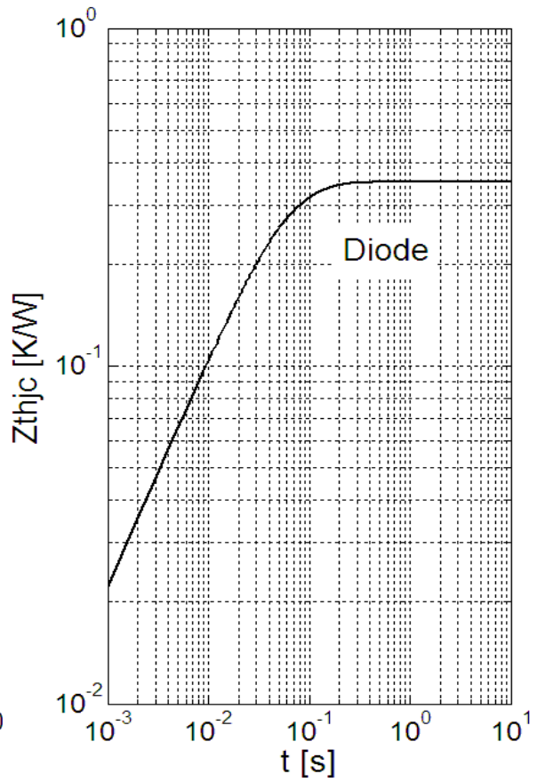
Fig 10. Diode Transient Thermal Impedance
