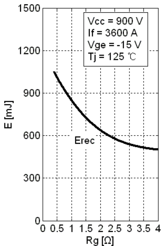
Fig 9. Diode Switching Loss vs. R_G
