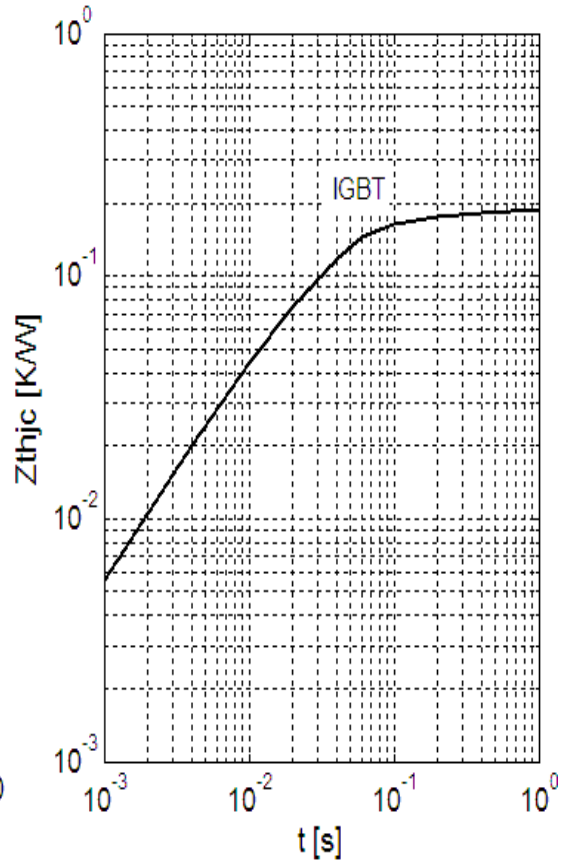
Fig 6. IGBT Transient Thermal Impedance
